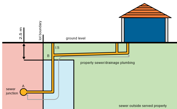
Diagram 8 Example of sewer arrangement
