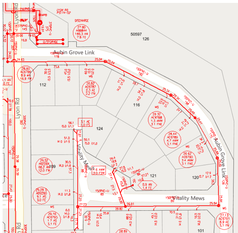
Diagram 5 BYDA sewer drawing.
