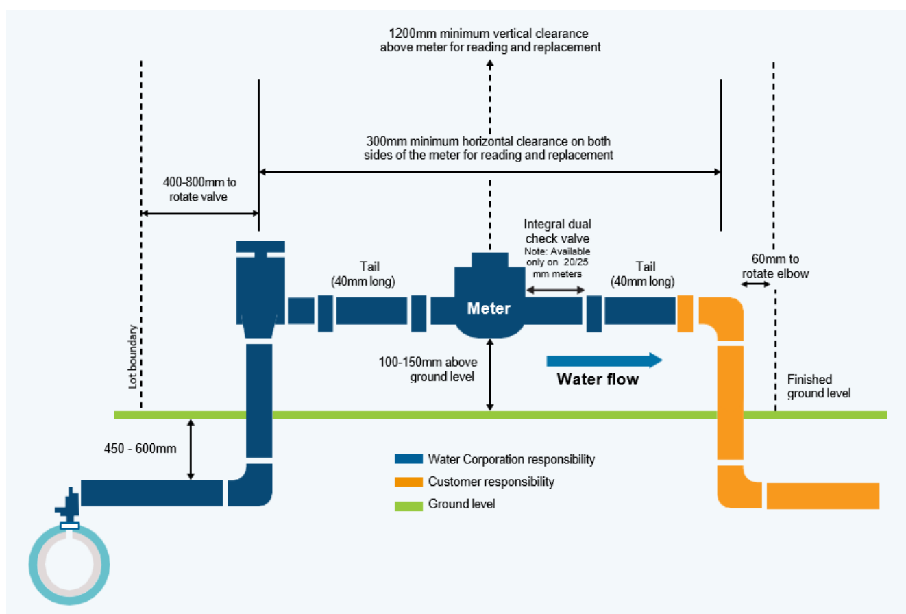
Diagram 10 20-25mm water meter with dual check valve arrangement
