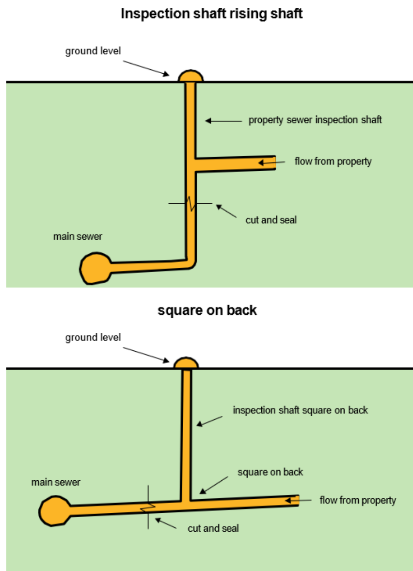
Diagram 7 Correct sewer disconnections.
