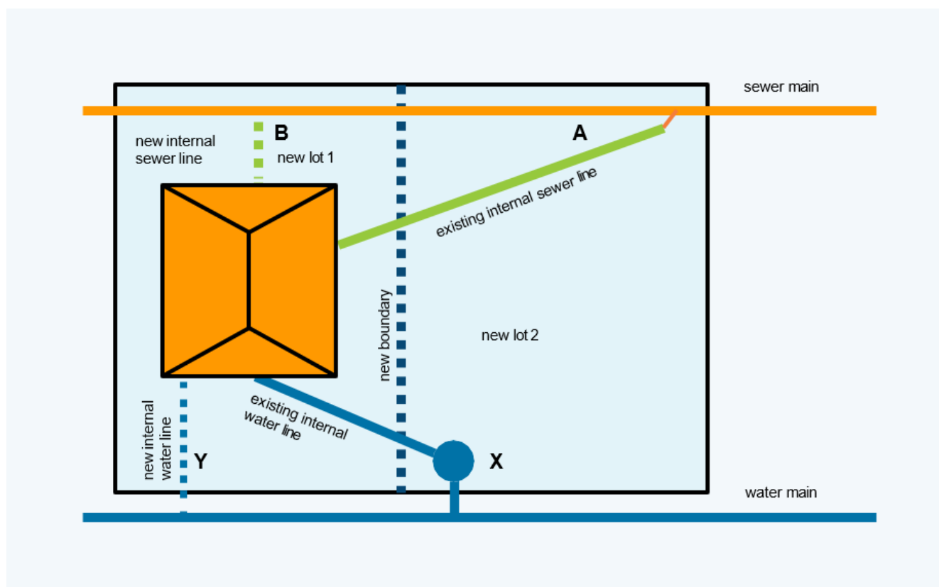
Diagram 9 Isolation of lines.
