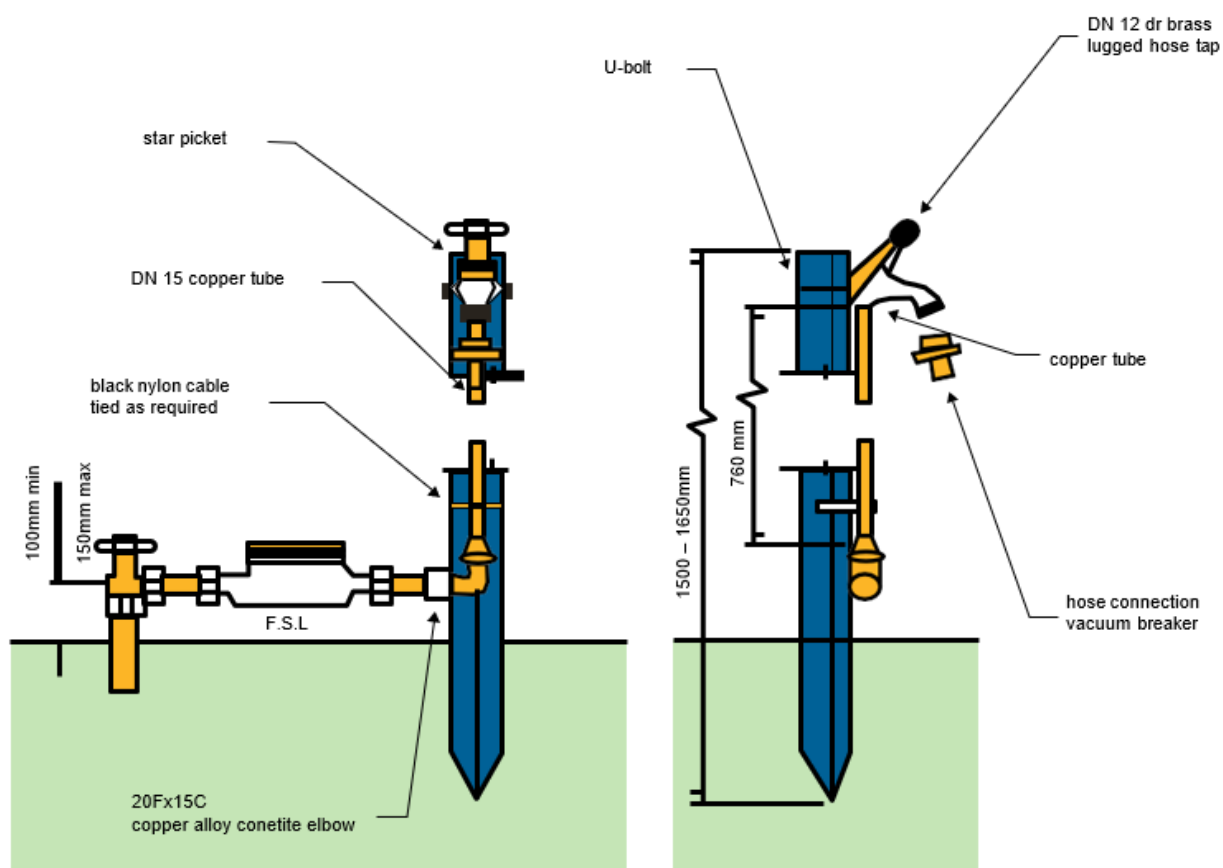
Diagram 6 Connection for temporary standpipe.
