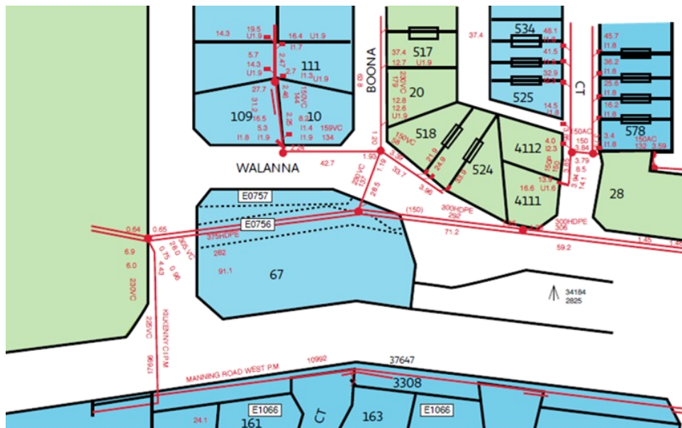
Diagram 4 BYDA Plan example with sewer lines.
