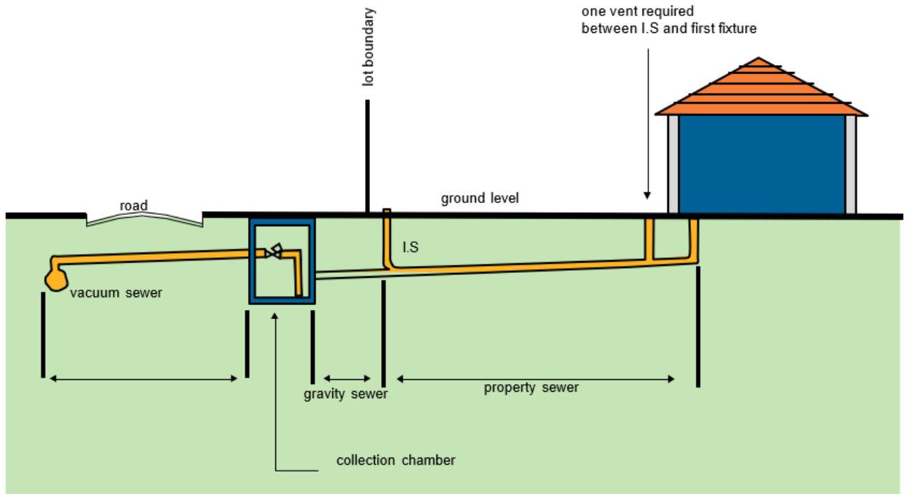
Diagram 1 Collection where collection chamber is located outside property boundary.
