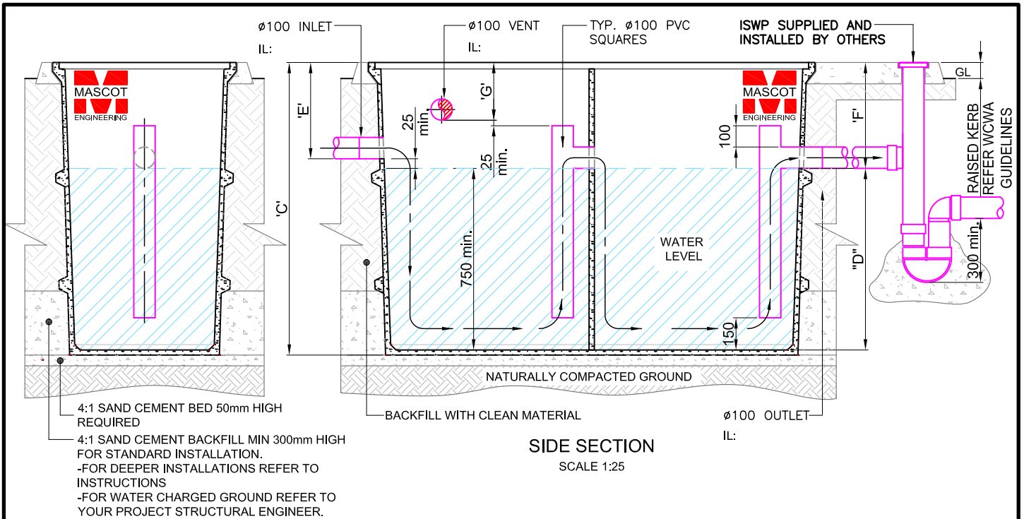
END SECTION SCALE 1:25
