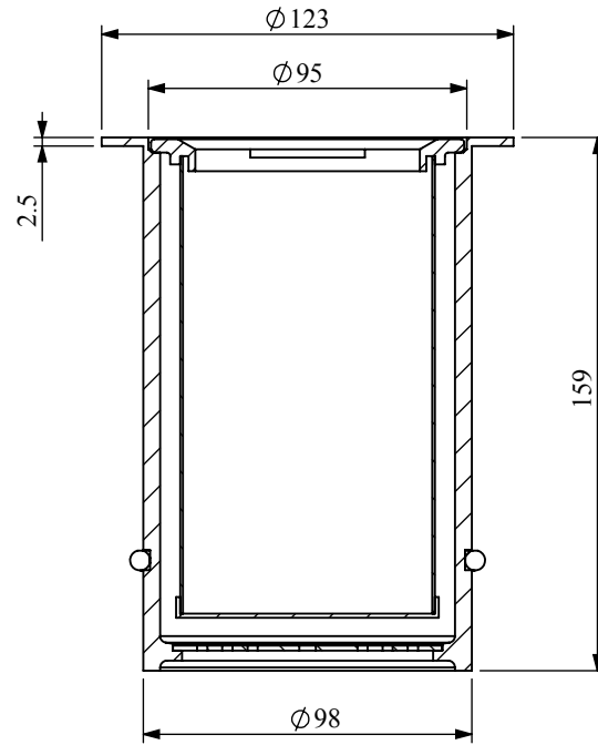
SECTION C-C SCALE 1 : 2.5
