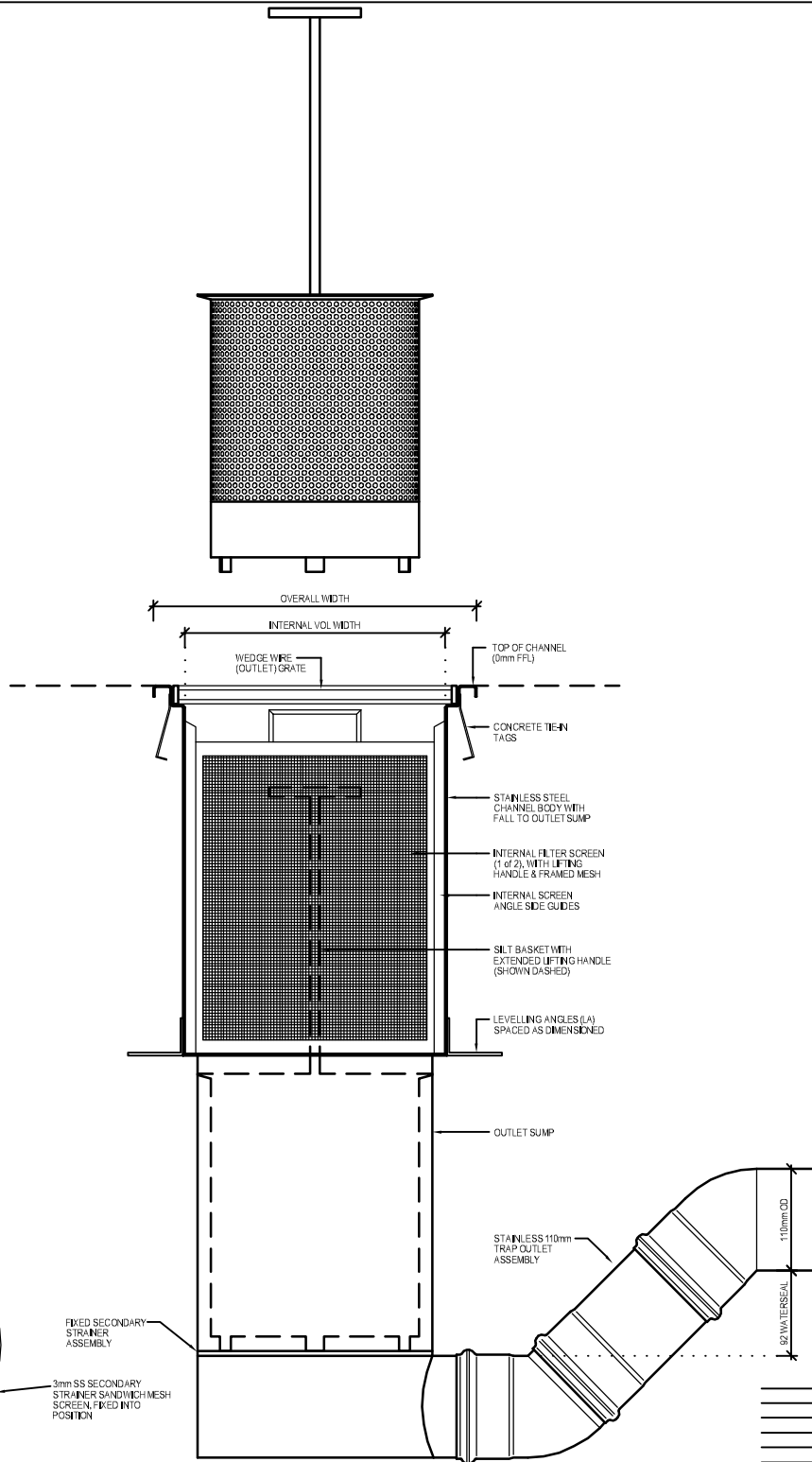
SURGE CHANNEL END: OUTLET DETAIL (COMMON) AUSPRESS CHANNEL
