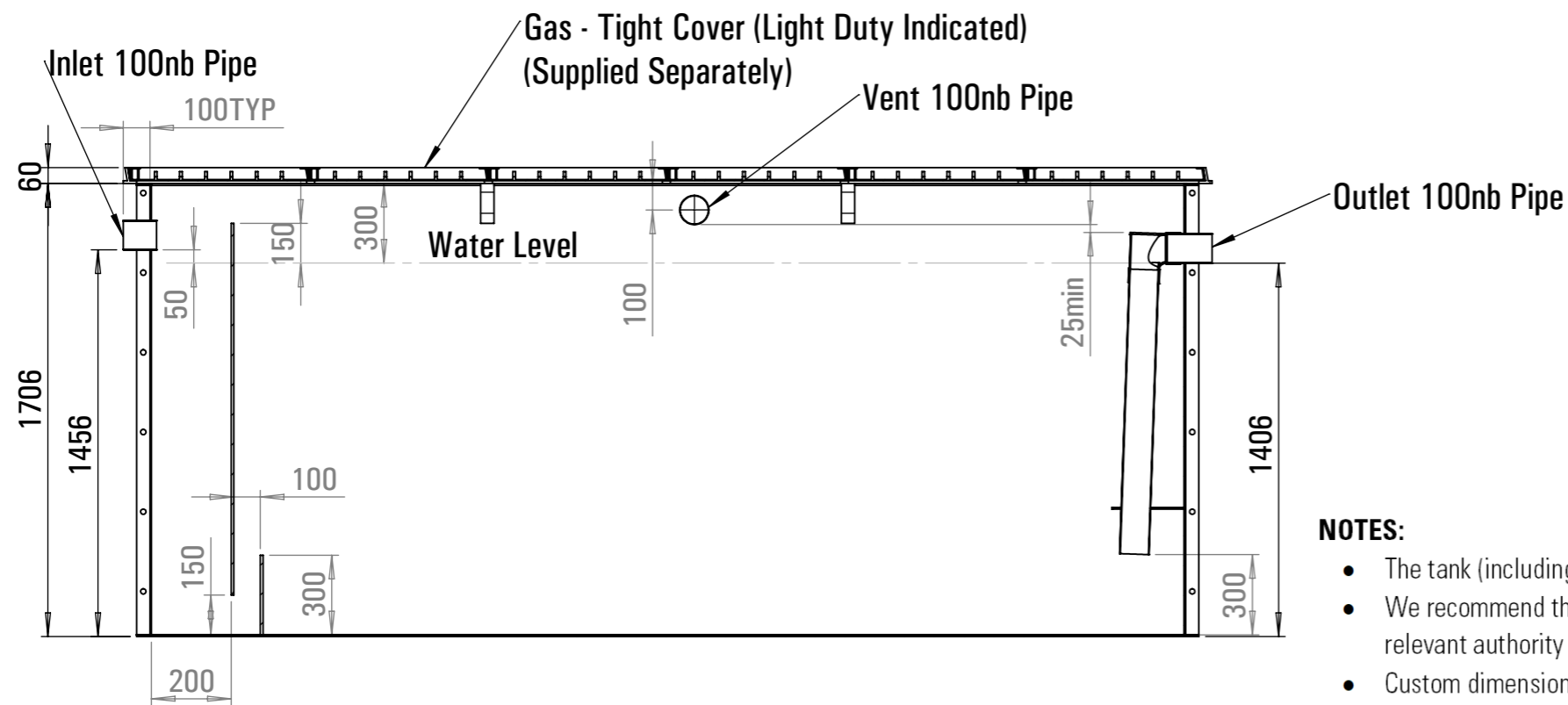
SECTION B-B
