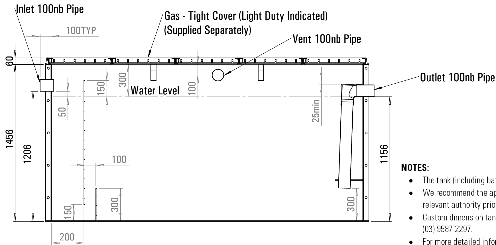
SECTION B-B
