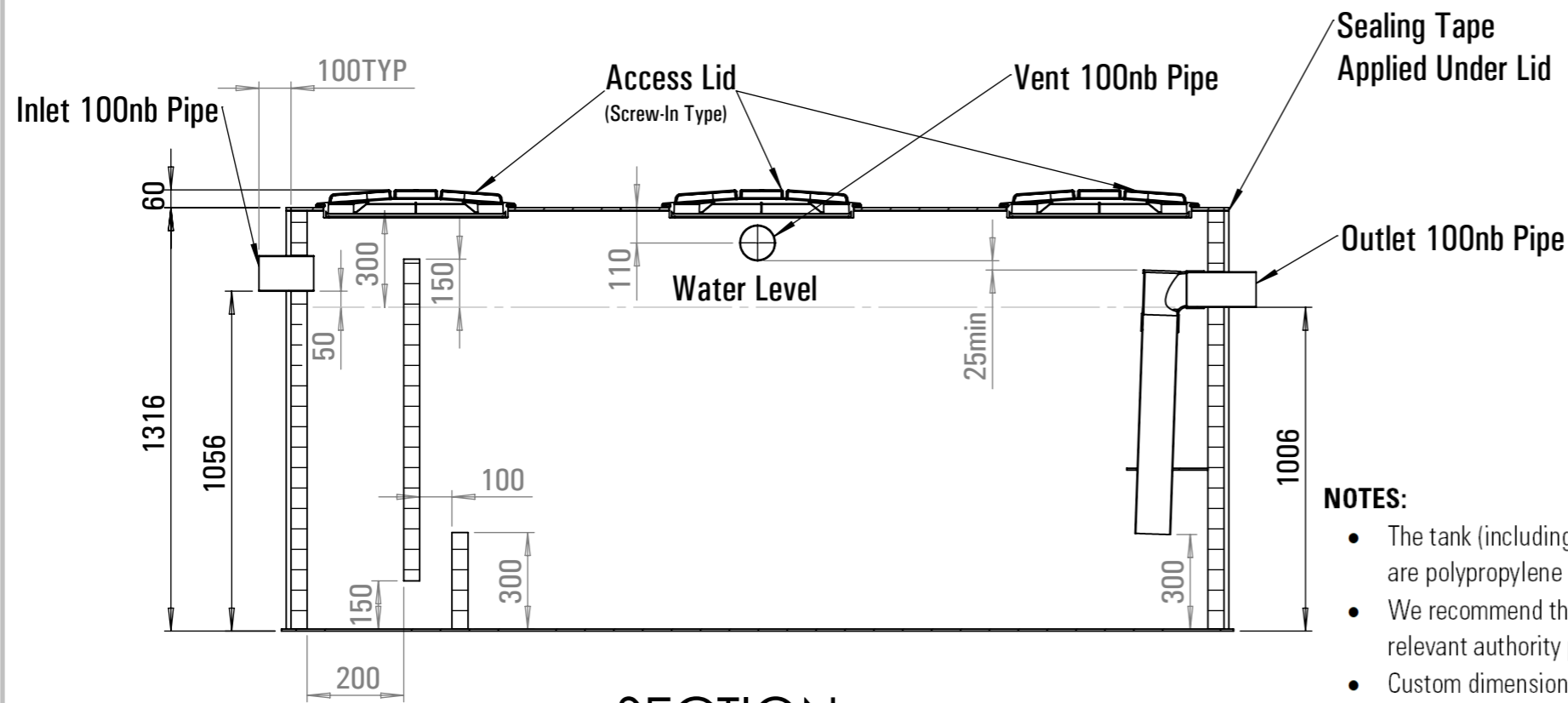
SECTION B-B
