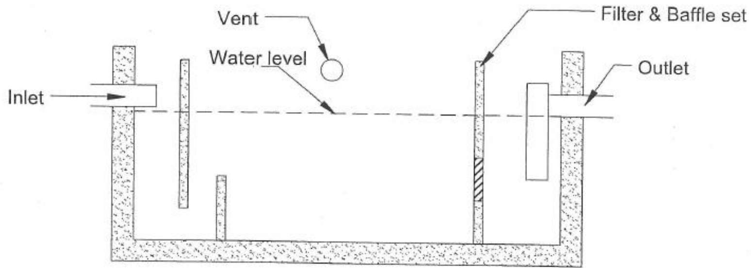
Side Section
