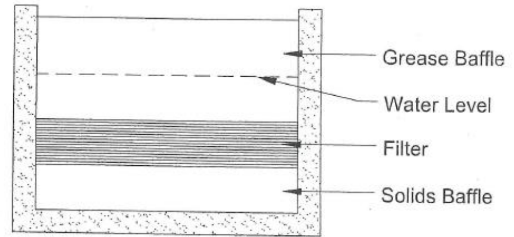
End Section
