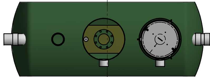
PART PLAN (FILTER AND VALVE REMOVED FOR CLARITY)
