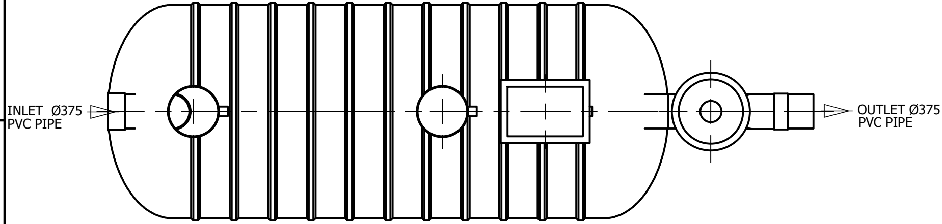
PLAN VIEW
