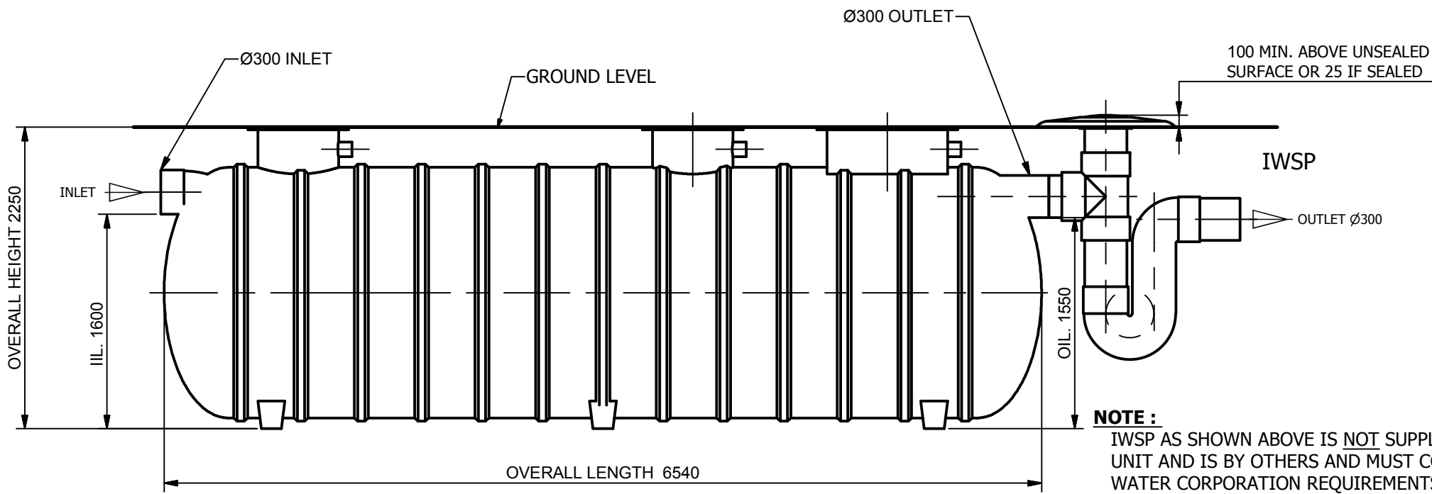
ELEVATION VIEW
