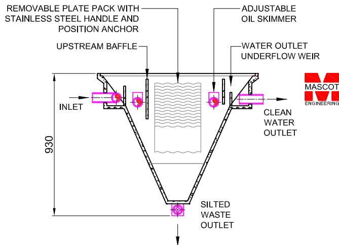
SIDE SECTION SCALE 1:25
