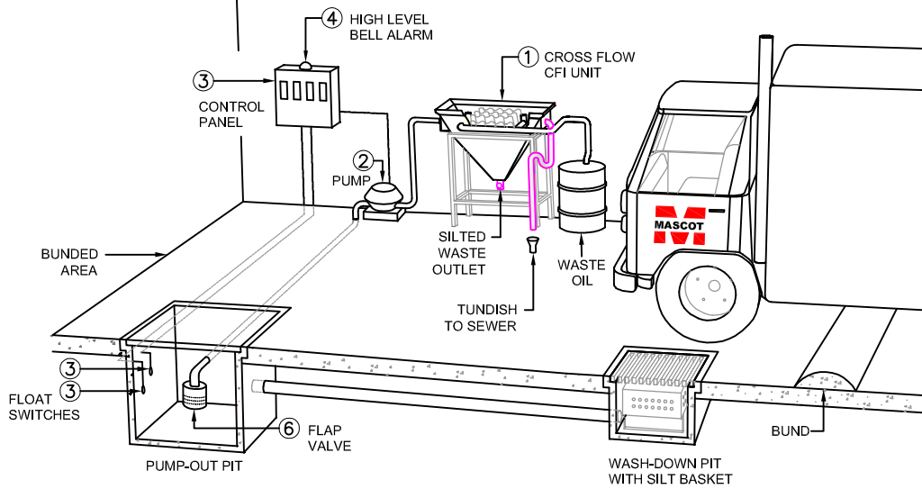
PICTORIAL VIEW OF SETUP SCALE: NTS
