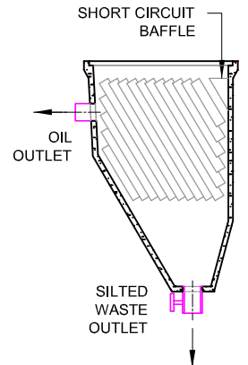
END SECTION SCALE 1:25
