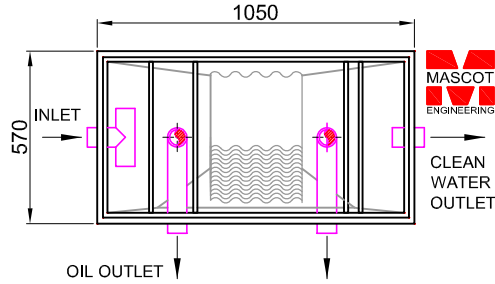
OPEN TANK PLAN VIEW SCALE 1:25
