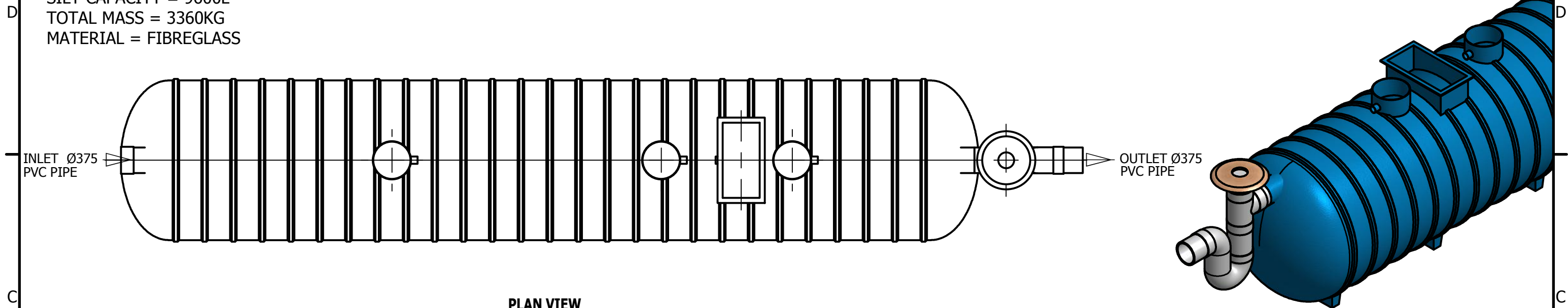
PLAN VIEW
