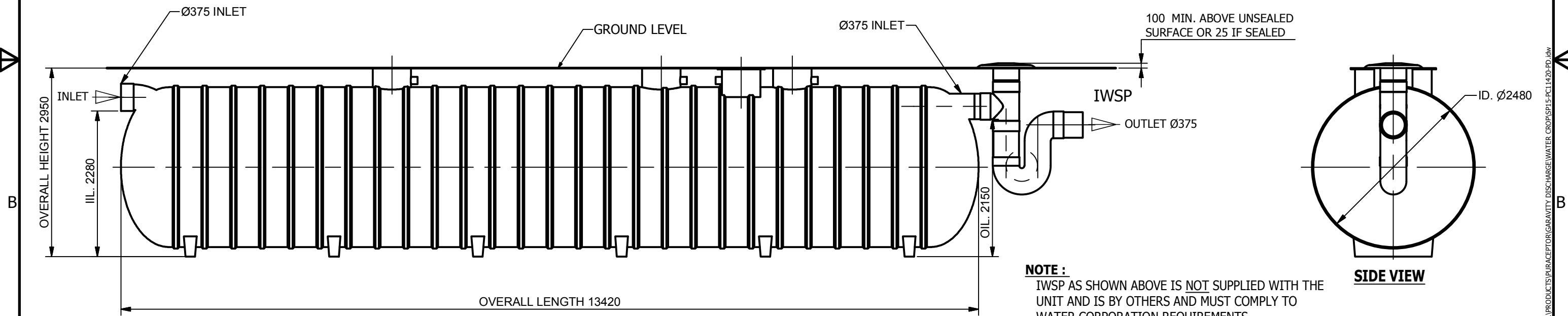
ELEVATION VIEW
