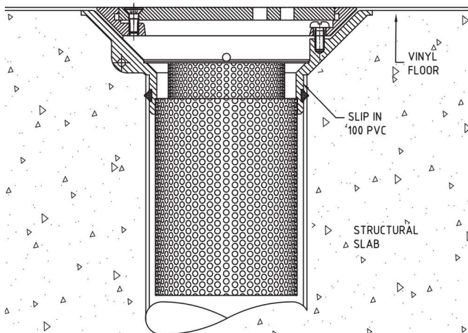
Slab On Ground
