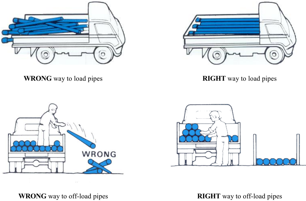
(a) Common (wrong and right) loading and off-loading arrangements for small pipe quantities
