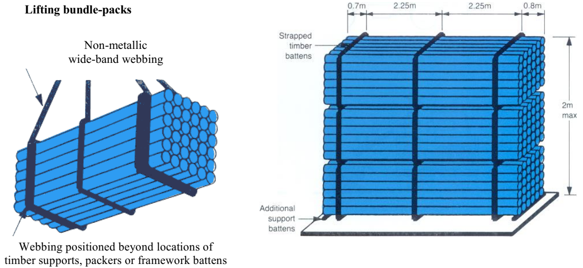
(a) Typical lifting and stacking arrangements for pipe bundles and crates
