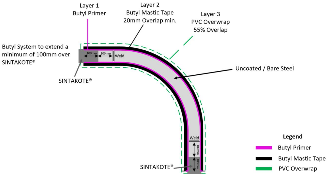
Figure 2: Butyl Wrap System
