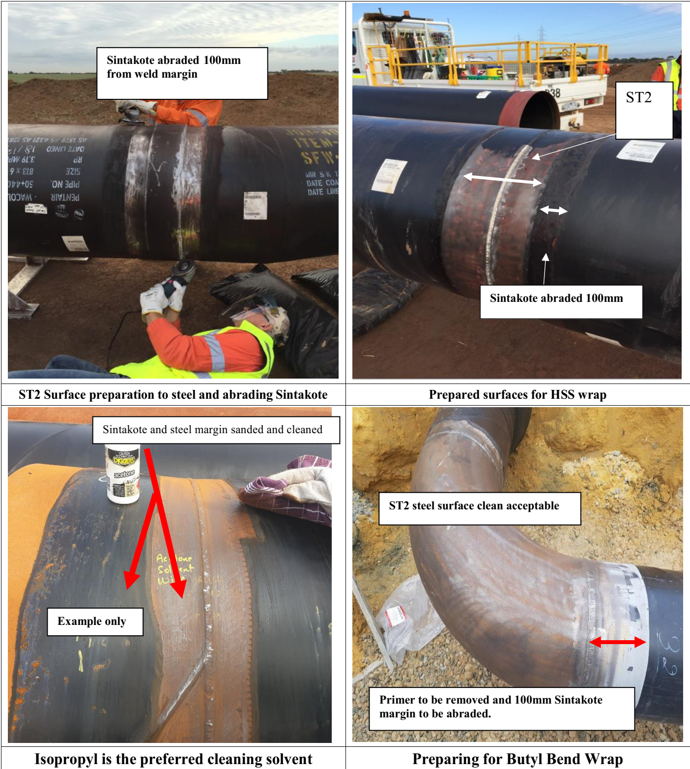
Figure 5: Sintakote & Steel Surface Preparation
