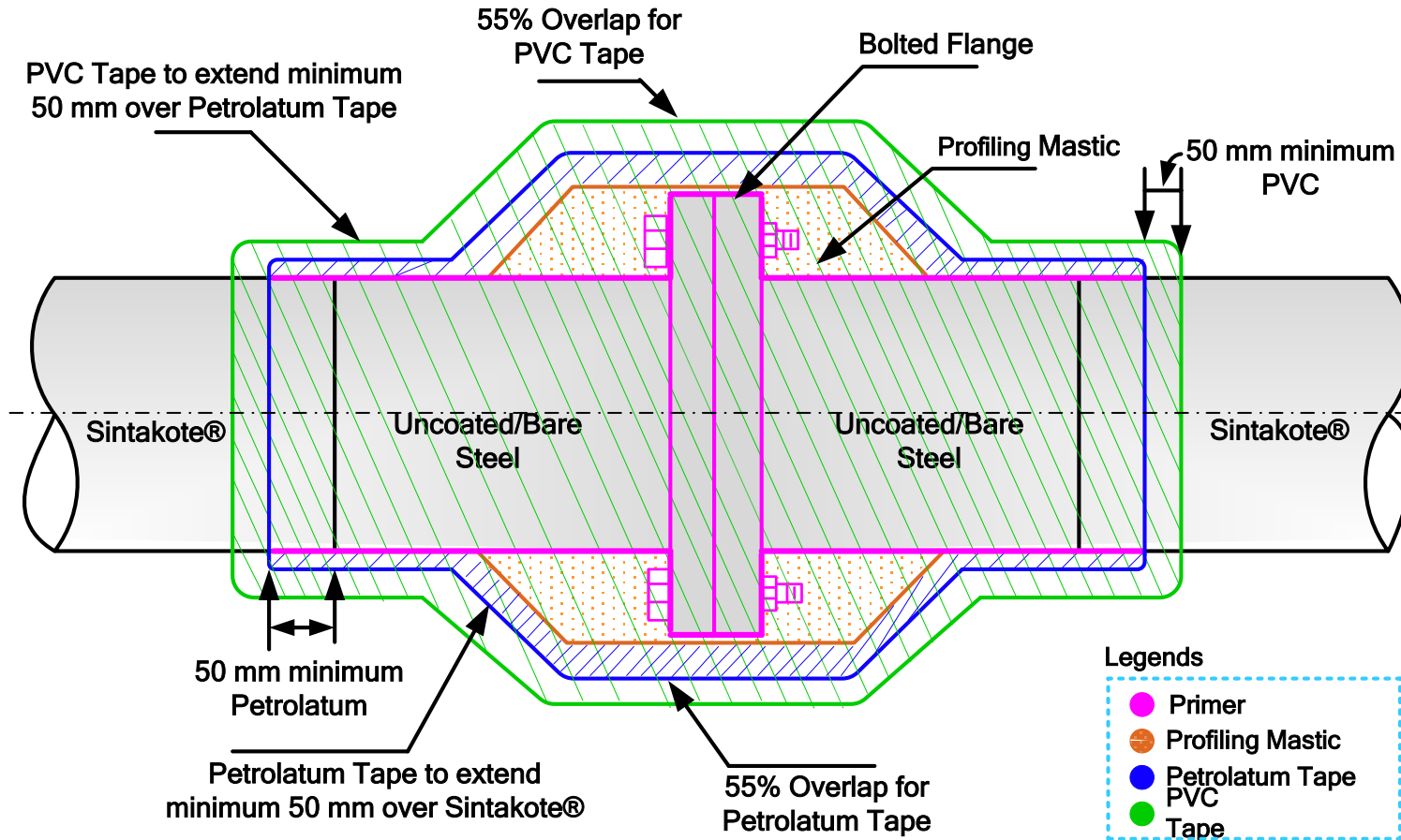
Figure 3: Petrolatum 4 Step System
