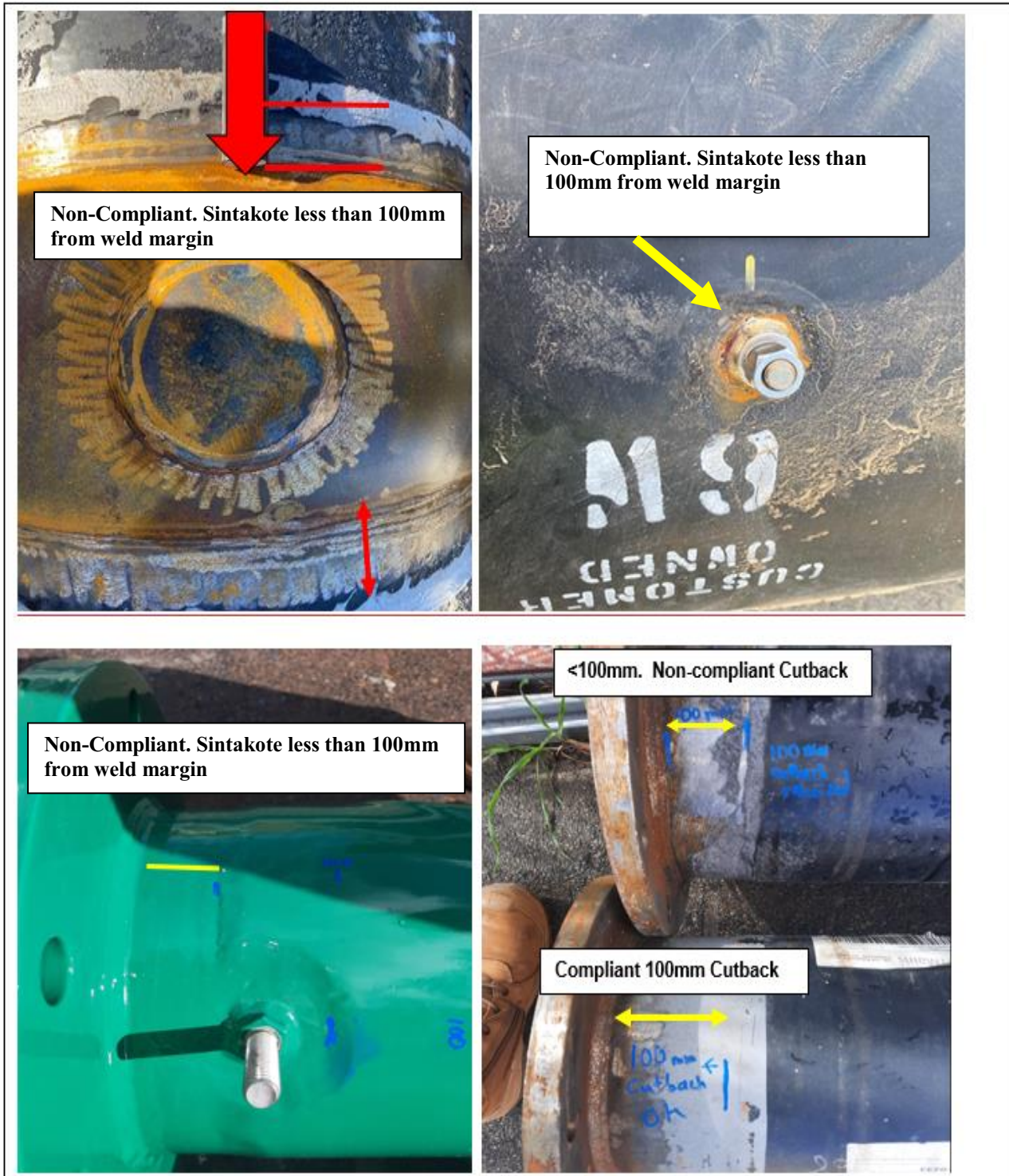
Figure 1: Sintakote to terminate a minimum 100mm from the weld zone as per AS4321
