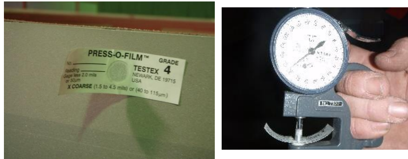
Figure 2: Blast Cleaned Surface Profile Measurement using TESTEX Tape
