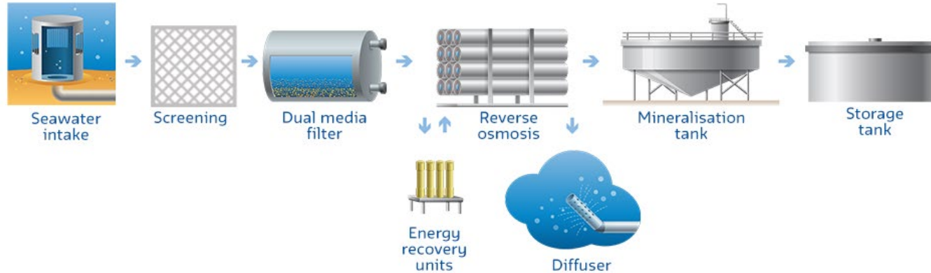
Figure 15: Typical desalination treatment process
