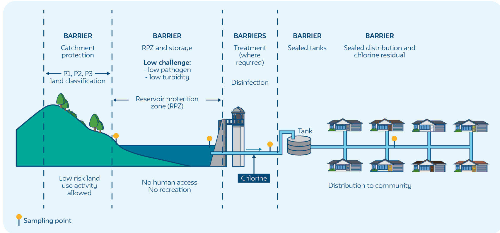
Figure 13: Surface water catchment – showing source (catchment) protection and additional multiple barriers
