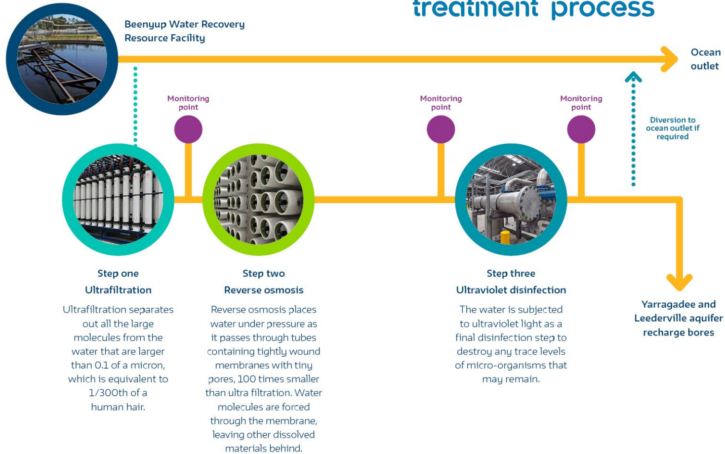
Figure 17: Advanced water treatment process
